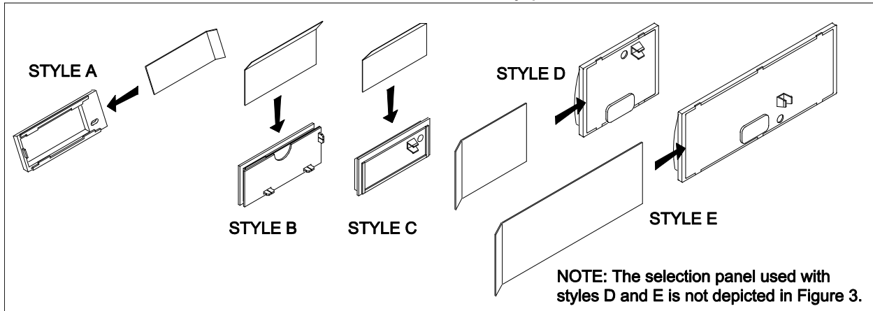
FIGURE 4 Part #1124016
