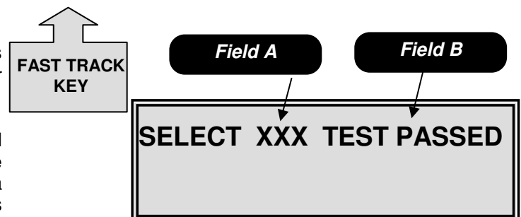
Mode 80 – Test Vend Field A is the item selection field. This field will be blank until a numeric key is pressed. Field B is the pass/fail field. If the motor passed it will read TEST PASSED if the motor failed it will read MTR ERROR.
