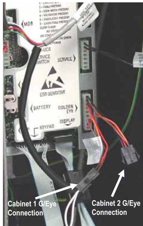
Photo 2 – Á LA CARTE Golden Eye connection in a 965 Tower using Cabinet 1
